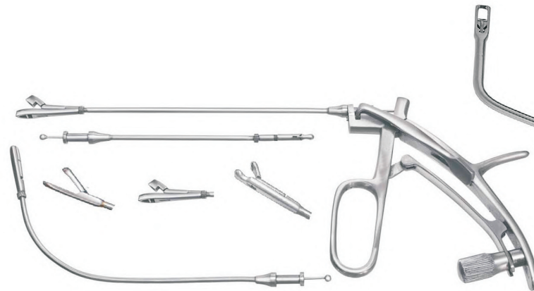
UNIVERSAL LARYNGEAL FORCEPS SET SI - 01155 .Tube with Atyle Straight Stiff 200mm .Tube with style Curved for Indirect Laryngeal Use 200mm .Laryngeal universal Cup Jaw .Laryngeal Biopsy .Laryngeal Cup Double side opening
